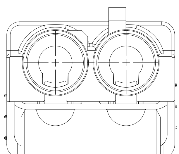
TYPE 105 SAME AS TYPE 101 EXCEPT AS SHOWN SCALE 4:1
