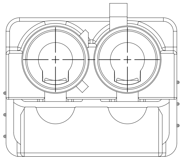
TYPE 108 SAME AS TYPE 101 EXCEPT AS SHOWN SCALE 4:1
