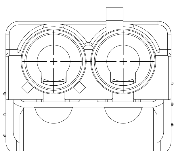
TYPE 110 SAME AS TYPE 101 EXCEPT AS SHOWN SCALE 4:1
