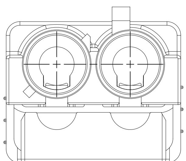
TYPE 109 SAME AS TYPE 101 EXCEPT AS SHOWN SCALE 4:1
