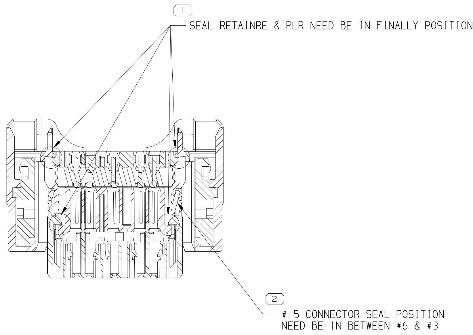
SECTION B-B
